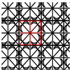
p4m
