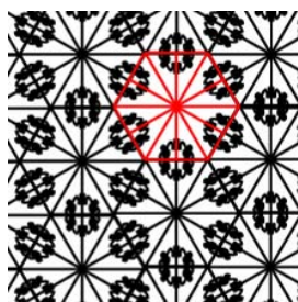
p6m
