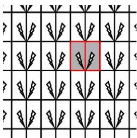
pm
