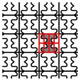
pmm
