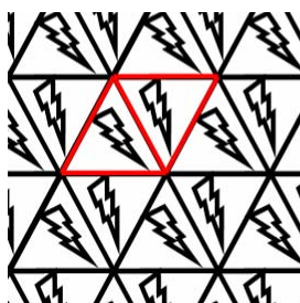
cm
