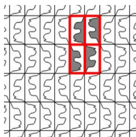
pgg
