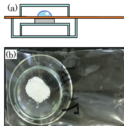
Figure 6. Equipment for measuring the permeability
